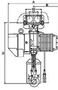
0.5 Ton - 5 Ton Electric Hoist With Trolley
