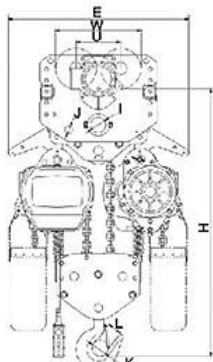
10 Ton Electric Hoist with Trolley
